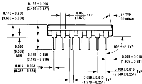
14-Lead Molded Dual-In-Line Package (N) Order Number DM74LS27N NS Package Number N14A
